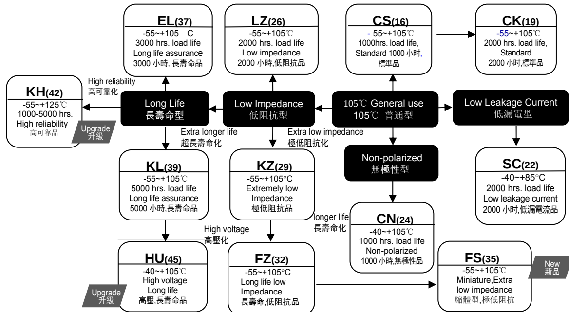
■ Chip Type Aluminum Electrolytic Capacitors 貼片式鋁電解電容器
